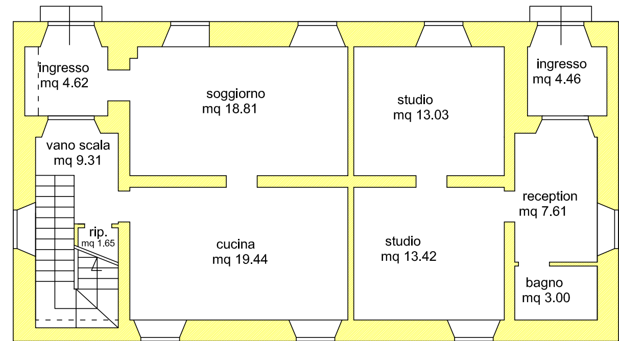
PIANO TERRA H = ml 3,00
