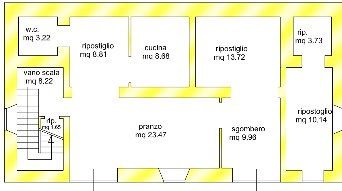
PIANO SEMINTERRATO H = ml 2,60
