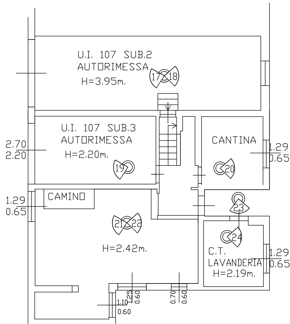
PIANO SEMINTERRATO
