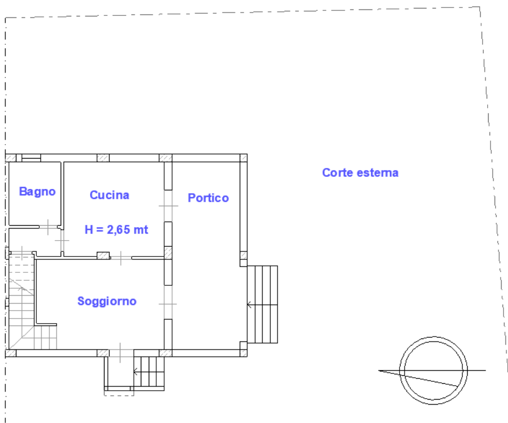
PIANO TERRA
