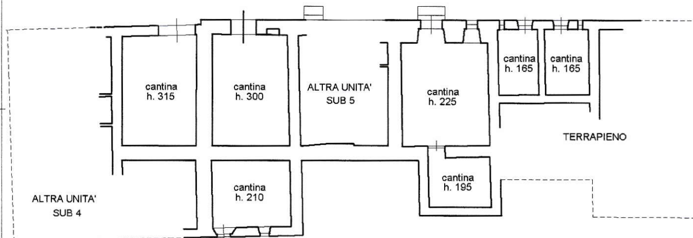
PIANO SEMINTERRATO
