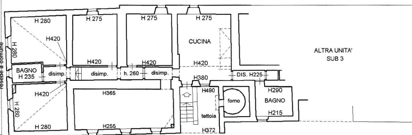
PIANO TERRA
