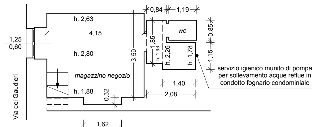
piano cantinato
