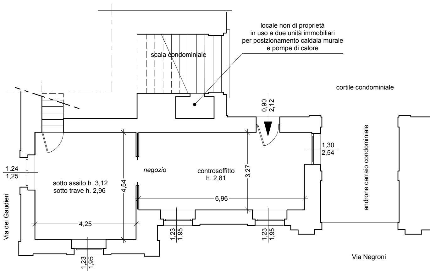
piano terra
