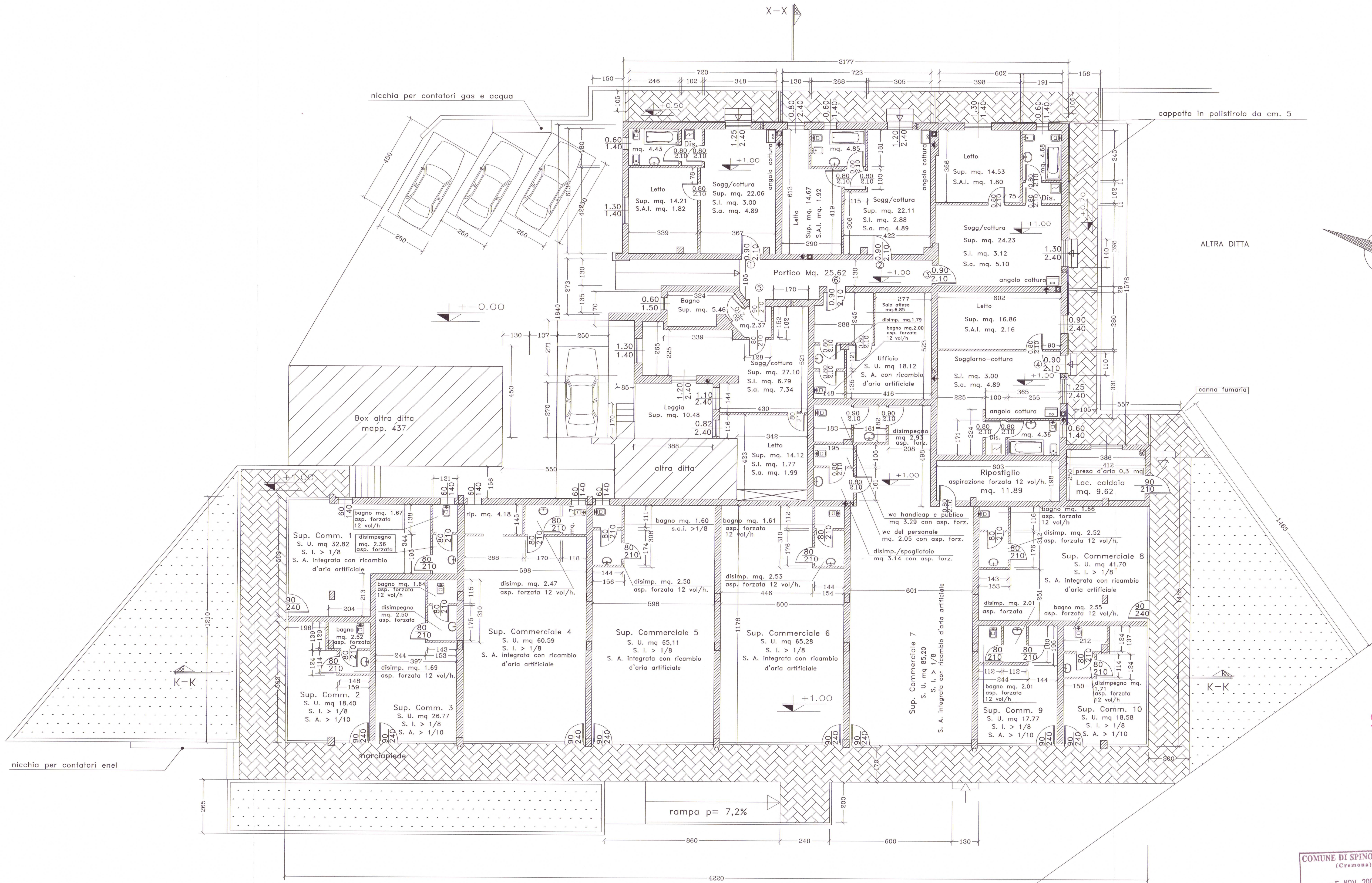
PIANTA PIANO TERRA (1:100)
