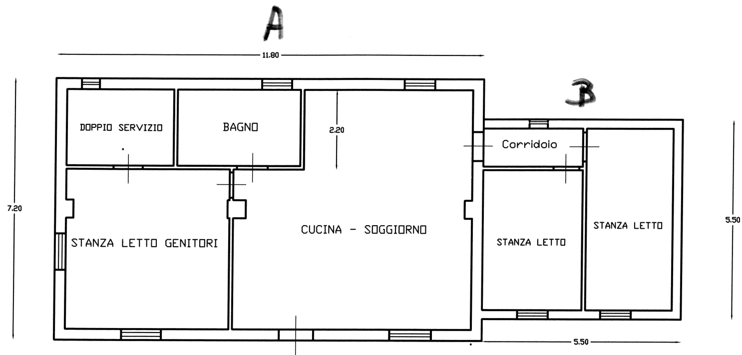
PIANO TERRA
