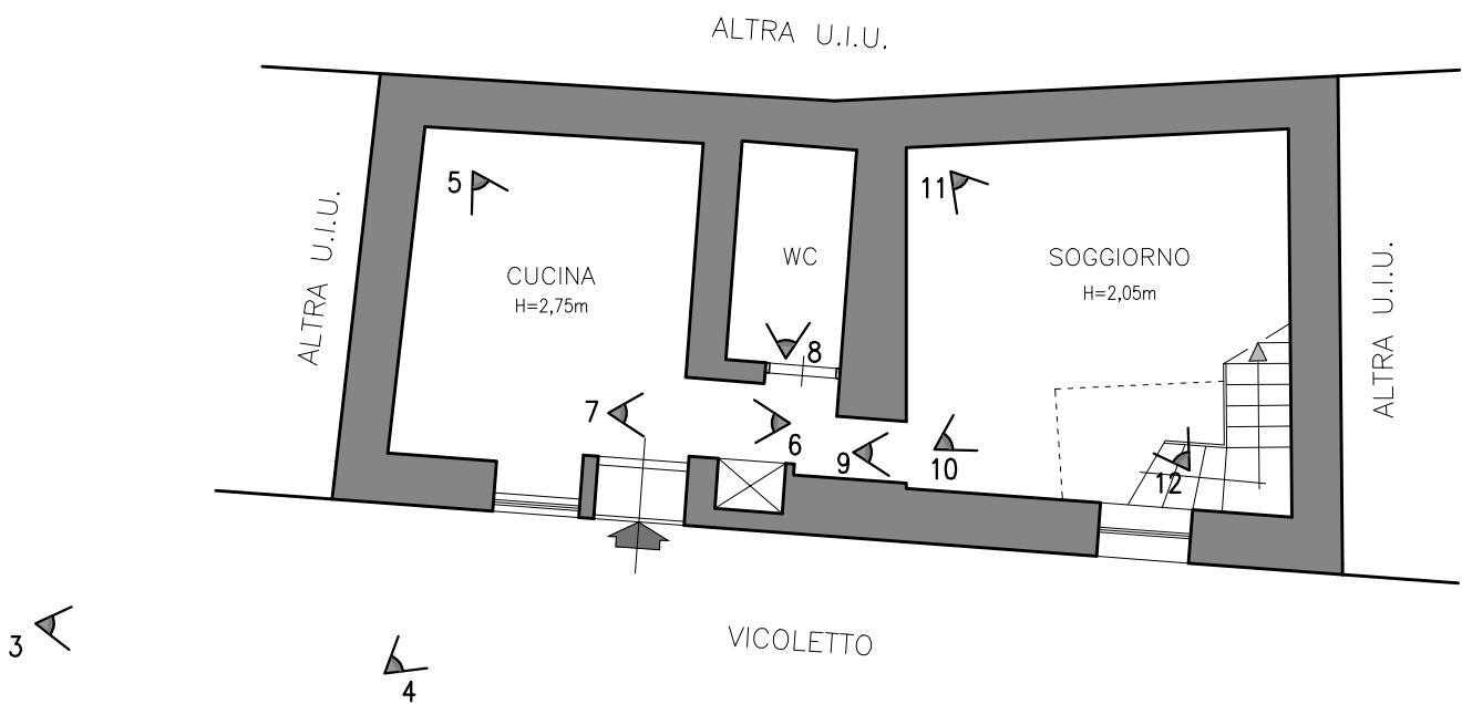
Piano Terra
