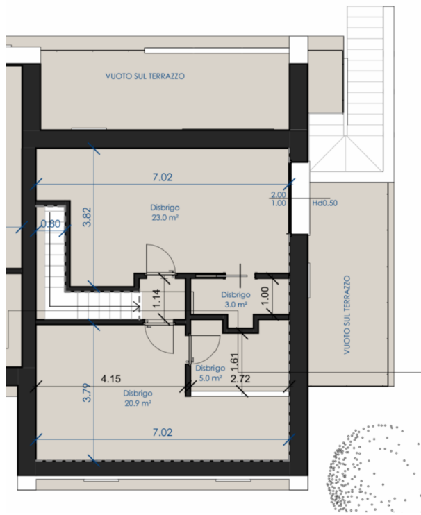
piano mansarda
