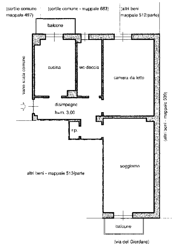
PIANO QUARTO
