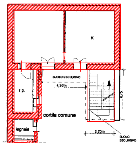
PIANO TERRA h=3,40
