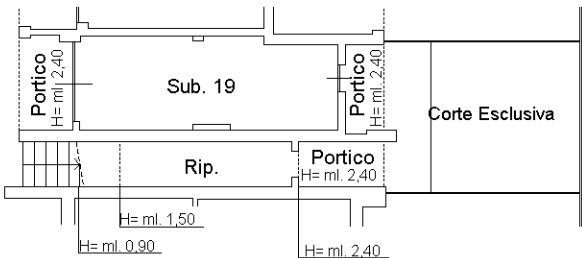
PIANO TERRENO
