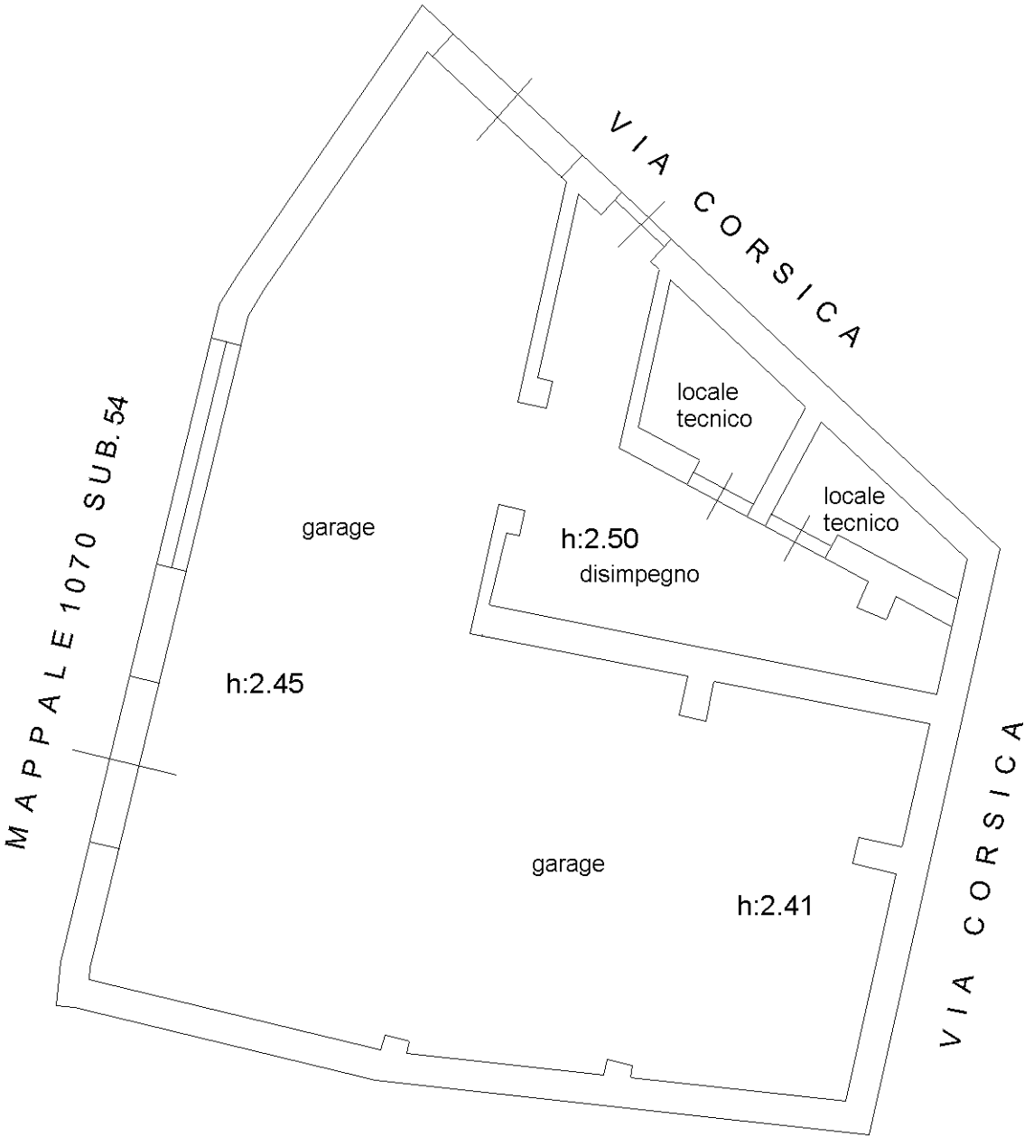
PIANO SEMINTERRATO
