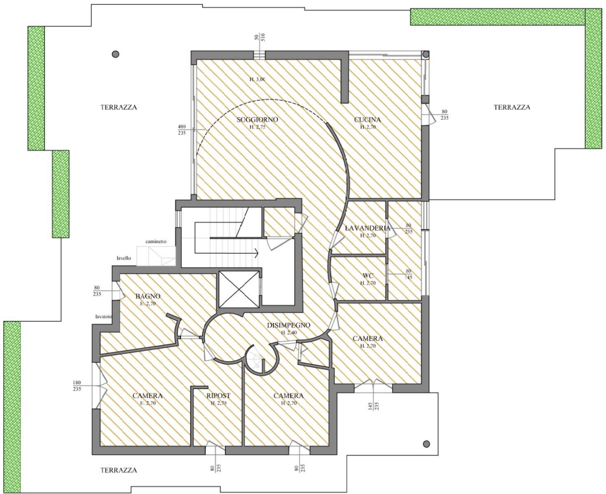
PIANO QUINTO
