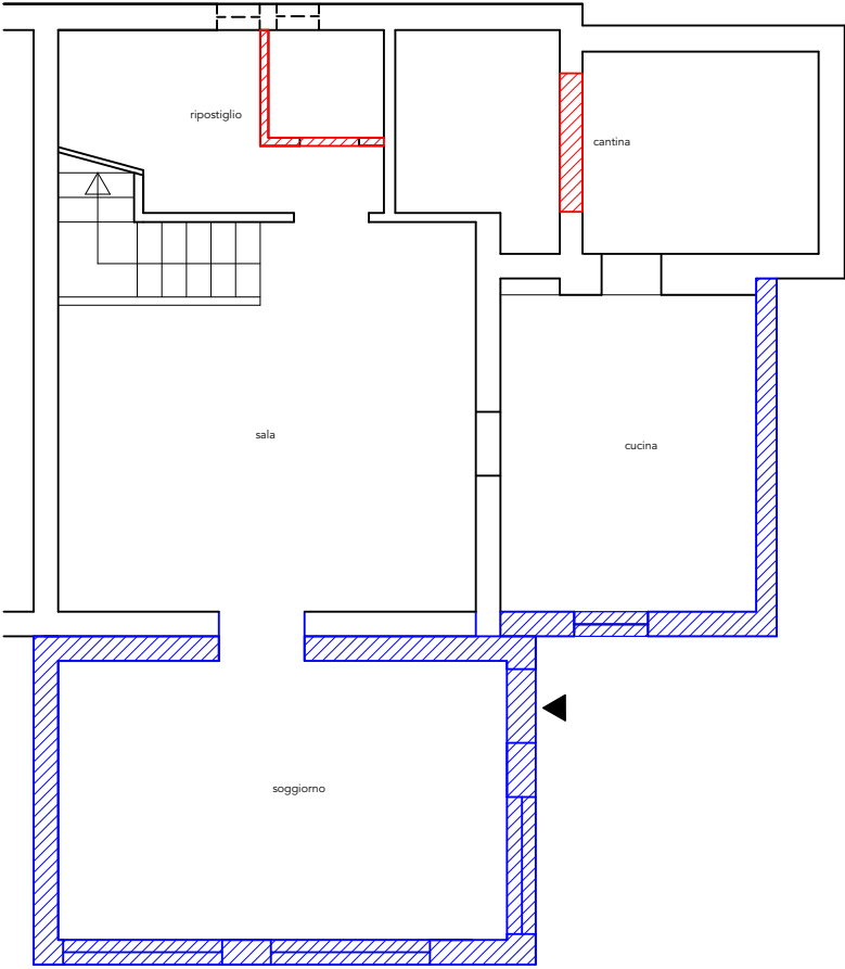
PIANO SEMINTERRATO H 285 cm
