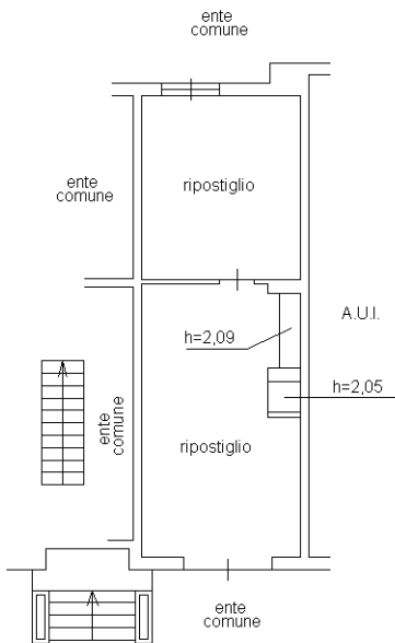
PIANO TERRA h=2,38
