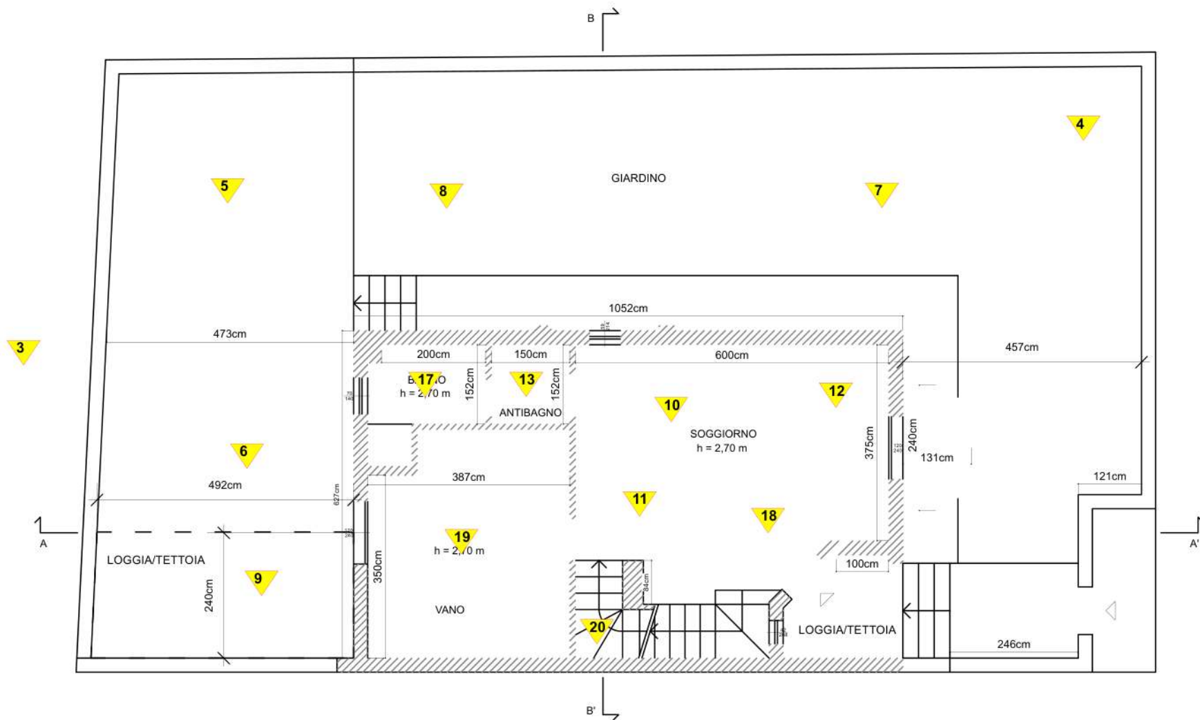
PIANO TERRA
