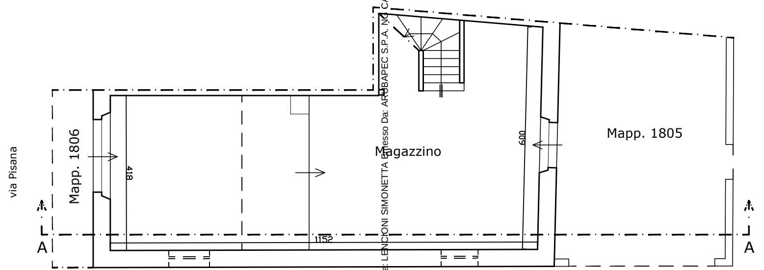
PIANO TERRA
