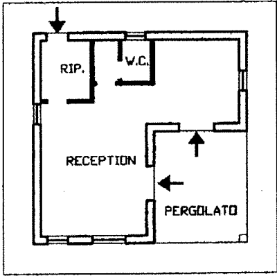
PIANO TERRA h = 3.95
