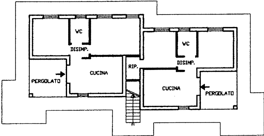
PIANO TERRA h= 3,13
