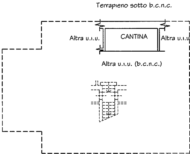
PIANO INTERRATO
