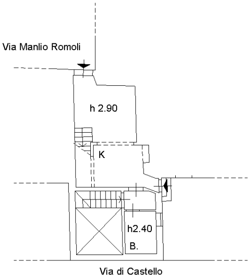
PIANO TERRENO
