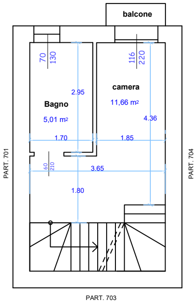
PIANO PRIMO H 2,50m
