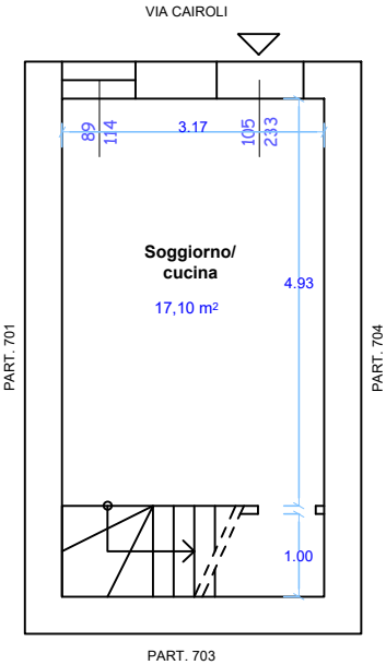
PIANO TERRA H 2,55m
