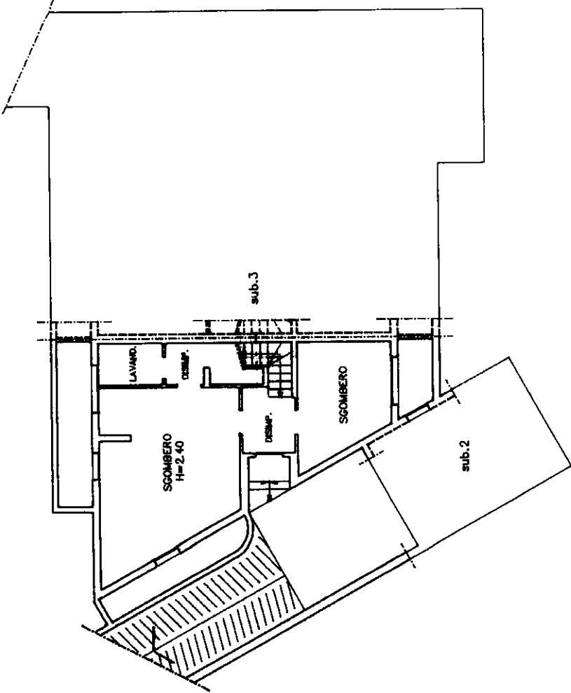
PIANO INTERRATO
