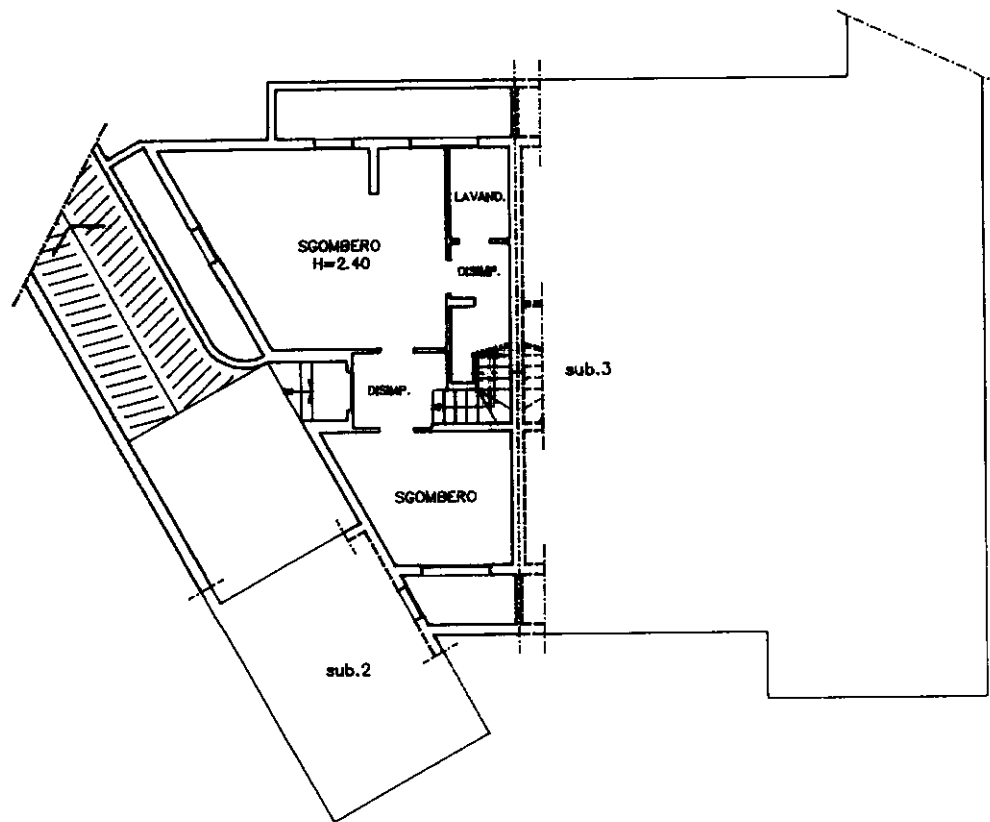
PIANO INTERRATO
