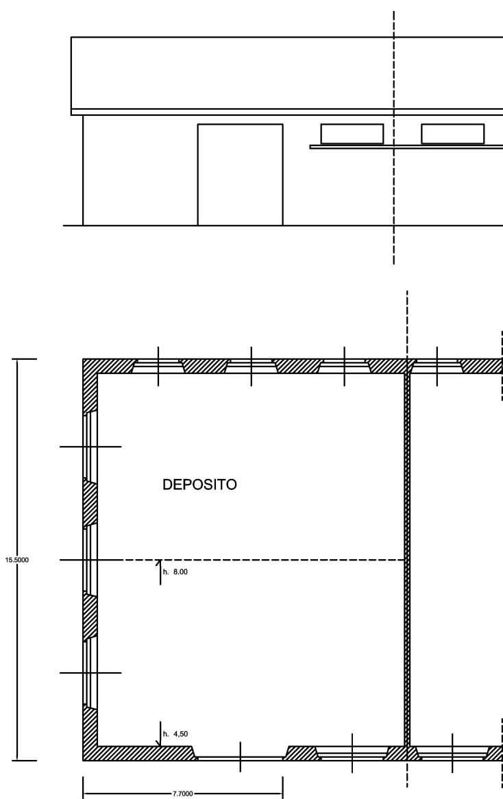
PIANO TERRA
