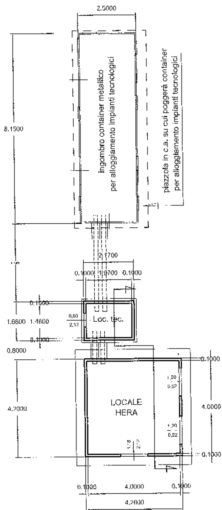
Piano Terra
