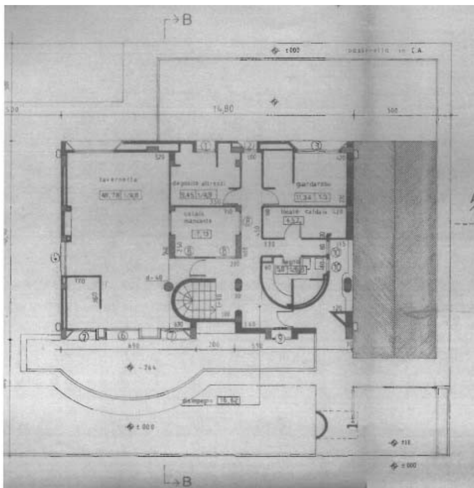
PIANO TERRA (variante a C.E. N°220/1989)
