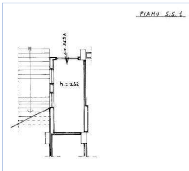
Planimetria Locle Deposito Piano S1 ( sub 16)
