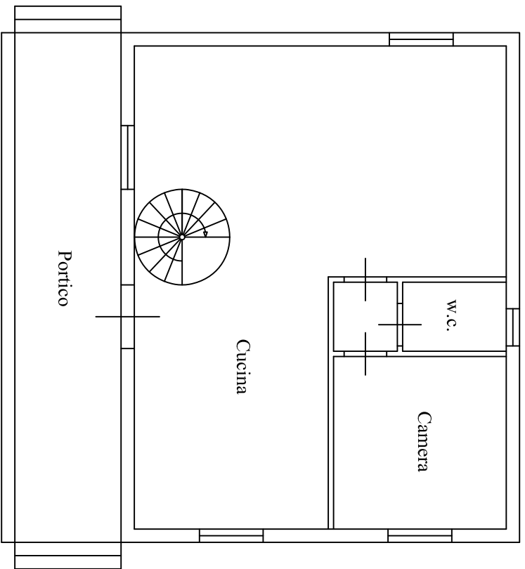
PIANO TERRA
