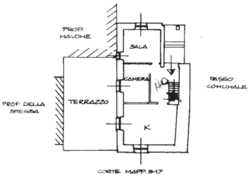
PIANO TERRA H=2.30
