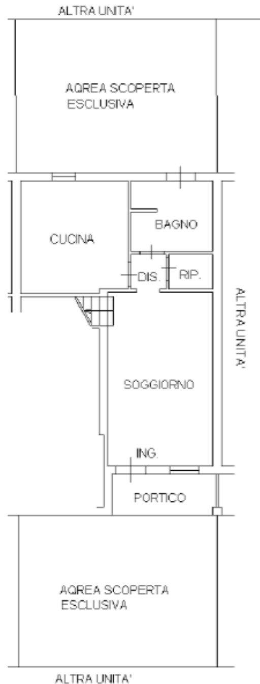
PIANO TERRA H=2.70
