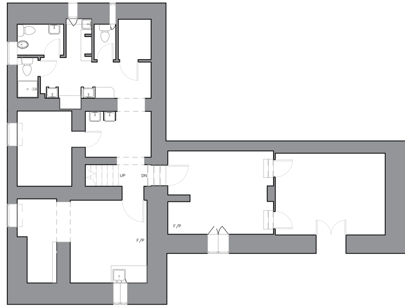
PIANO FONDI h 2,40-2,70
