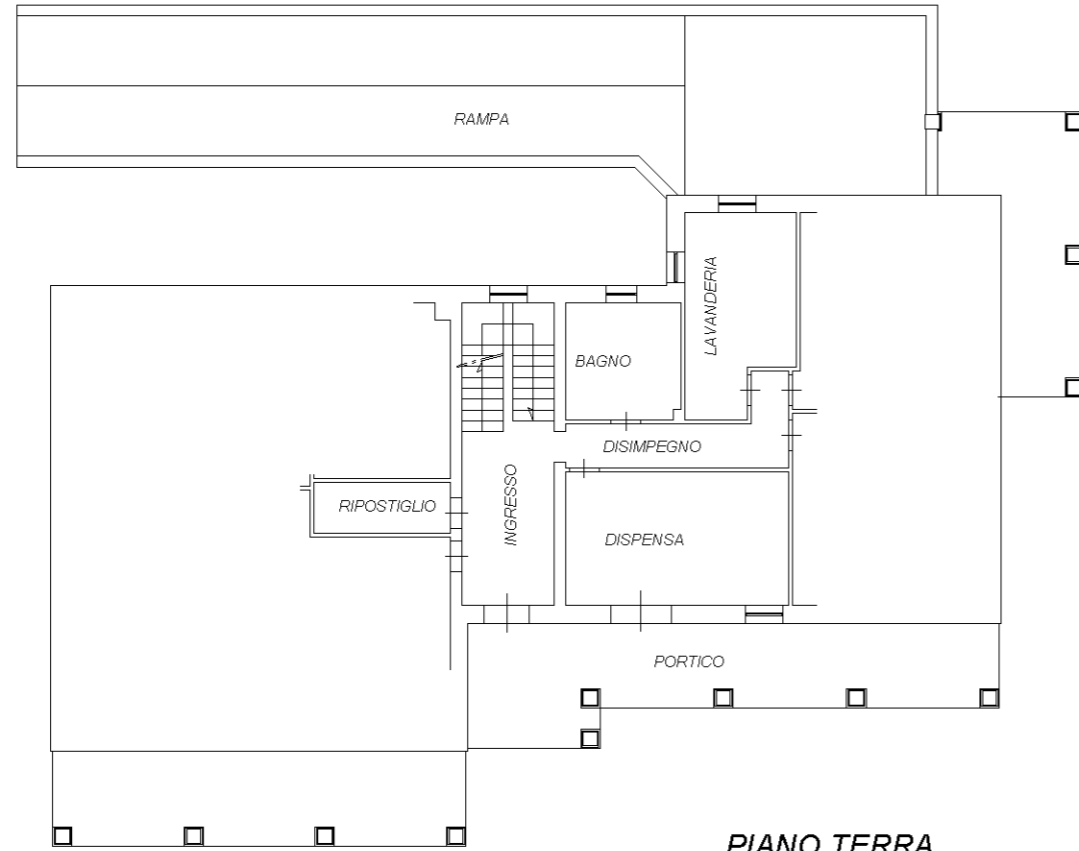
PIANO TERRA H=2.50
