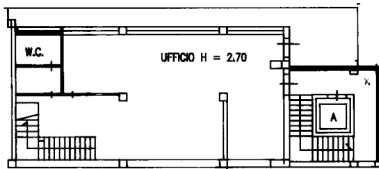
Piano terra
