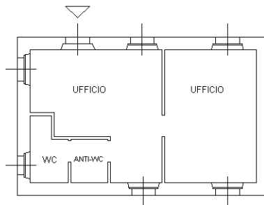
PIANTA PIANO TERRA H= 2,90m
