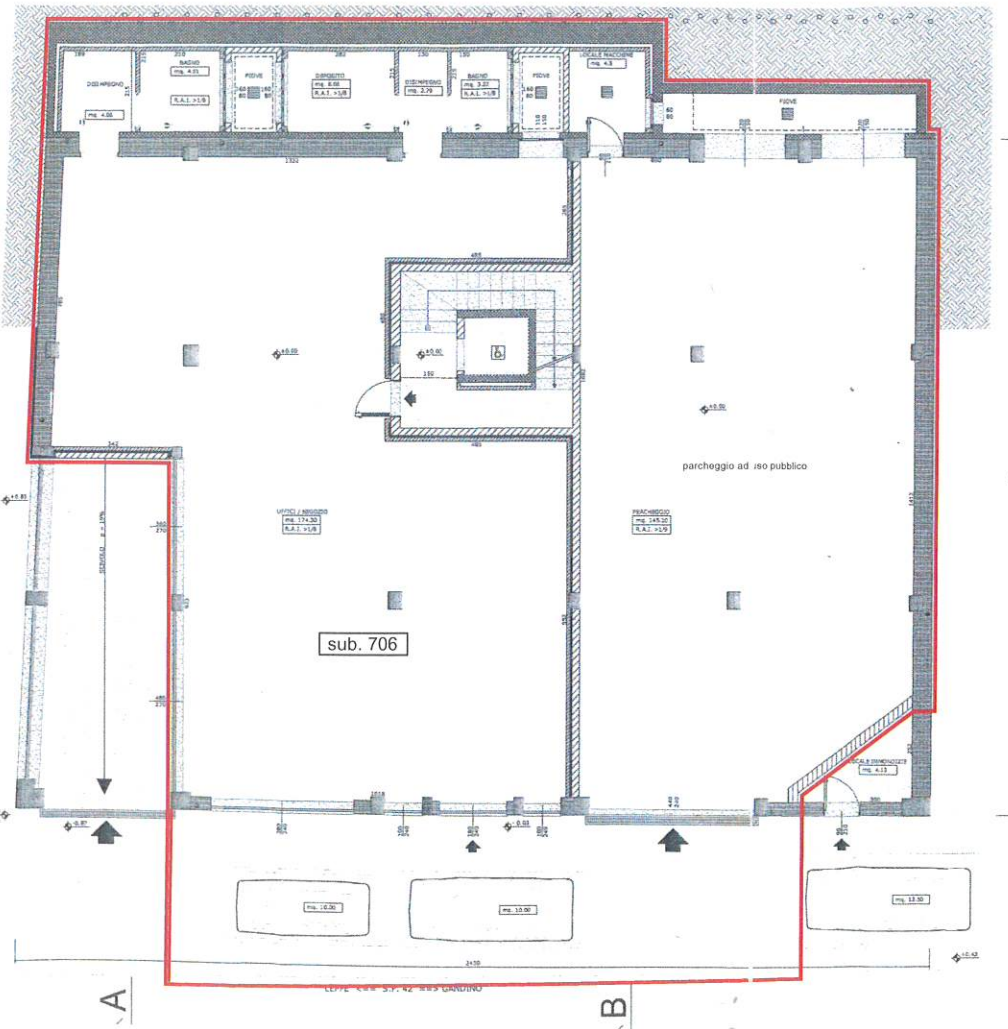
PIANO TERRA
