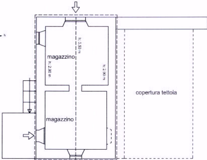
PIANO TERRA
