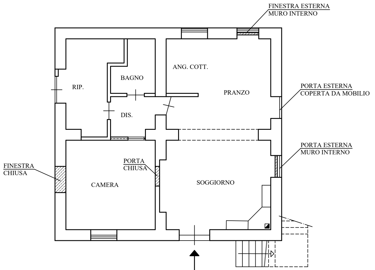
PLANIMETRIA PIANO TERRA
