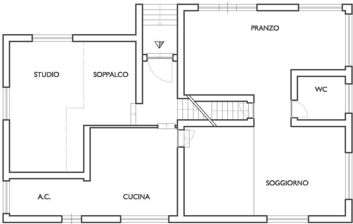
PIANO TERRA
