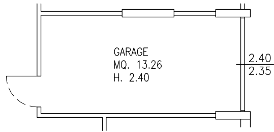
PIANO INTERRATO
