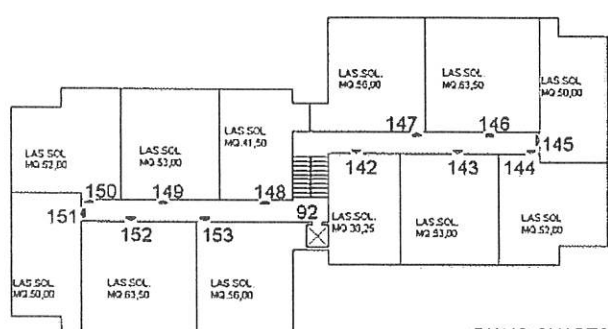
PIANO QUARTO
