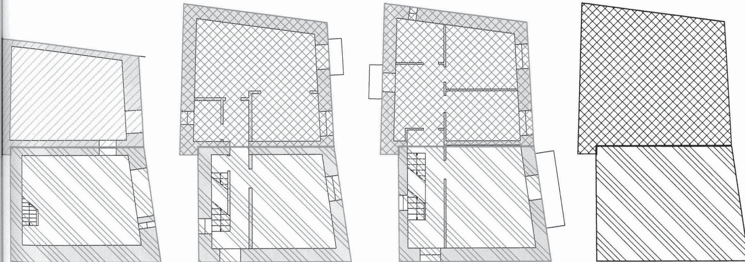
Piano seminterrato
