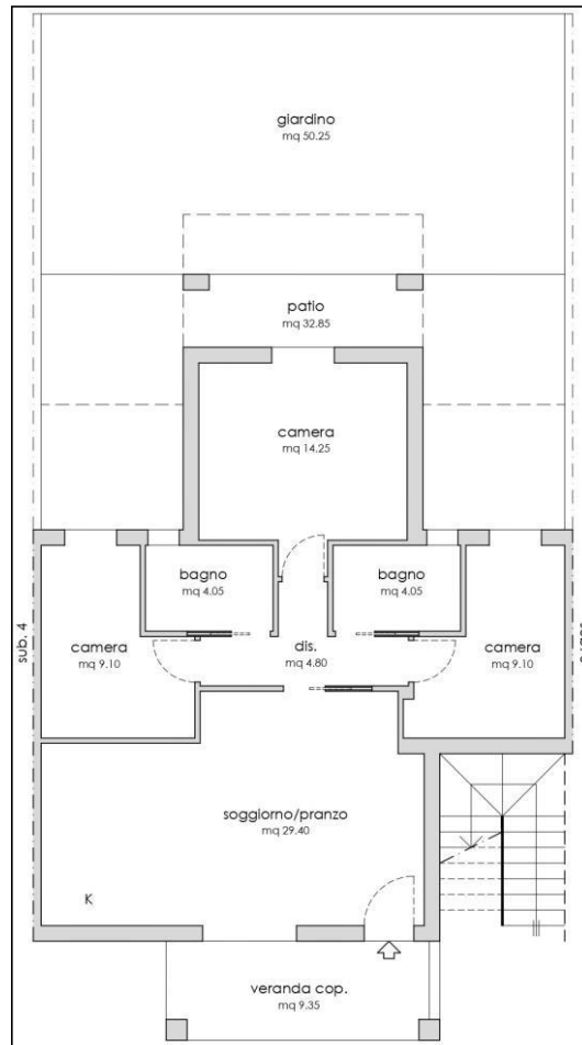
Pianta piano terra - Sub. 5
