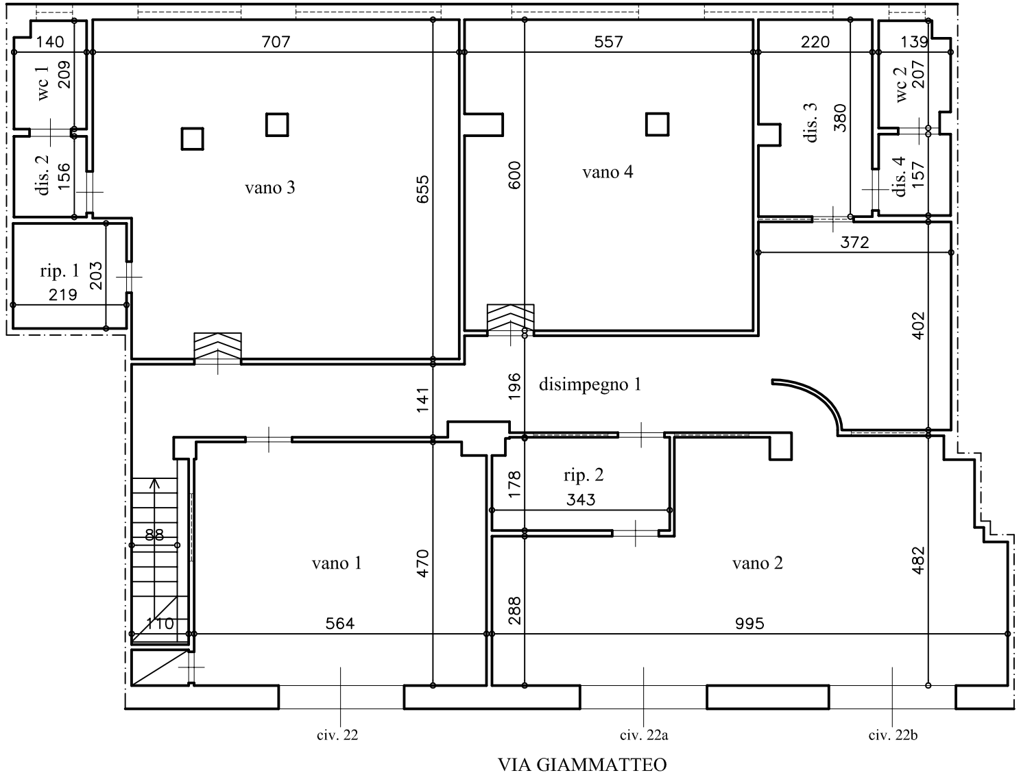
PIANTA PIANO TERRA h = ml 3.75
