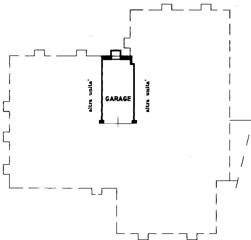
PIANTA PIANO INTERRATO h=2.40m
