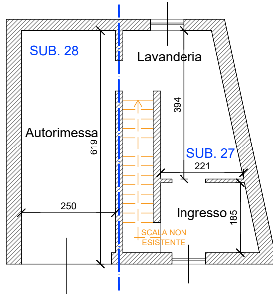
PIANO TERRA scala 1:100
