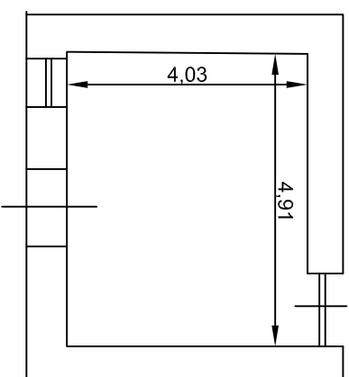
PIANO TERRA
