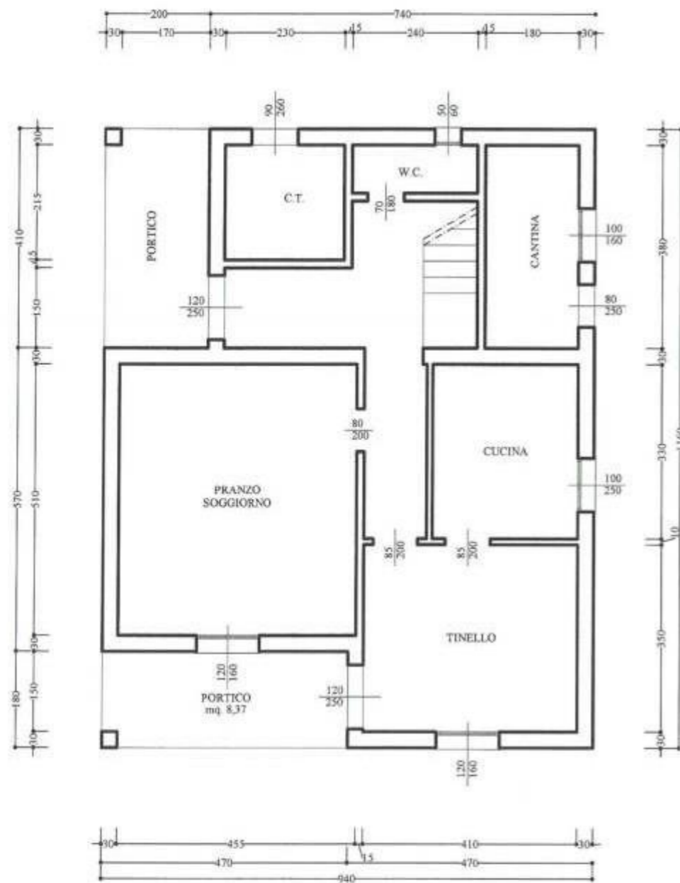
PIANO TERRA
