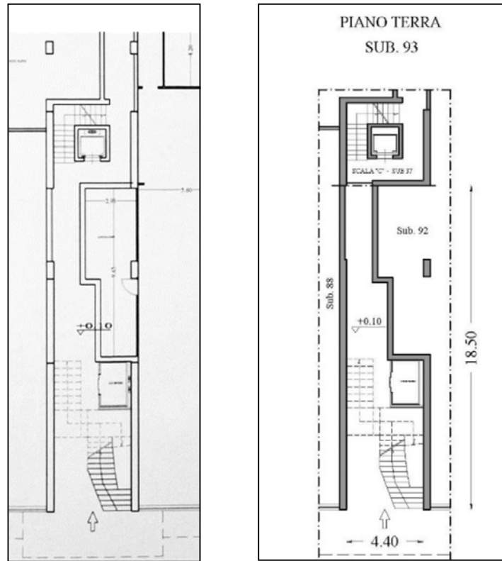
PIANO TERRA - CONFORME
