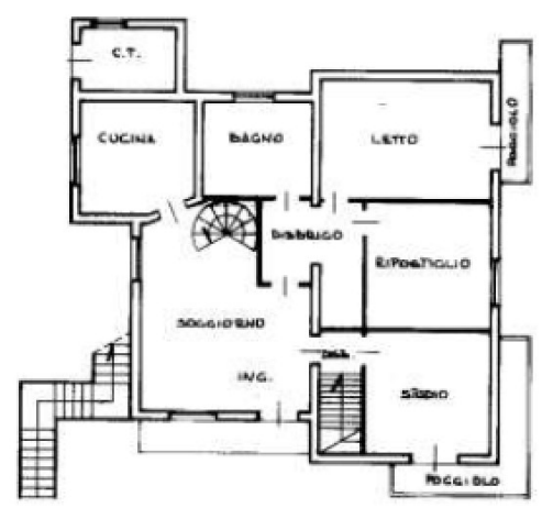
PIANTA PIANO TERRA Ha. 2,90 mt.
